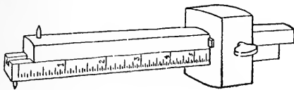
FIG. 34. MORTISE GAGE— DOUBLE BAR.
